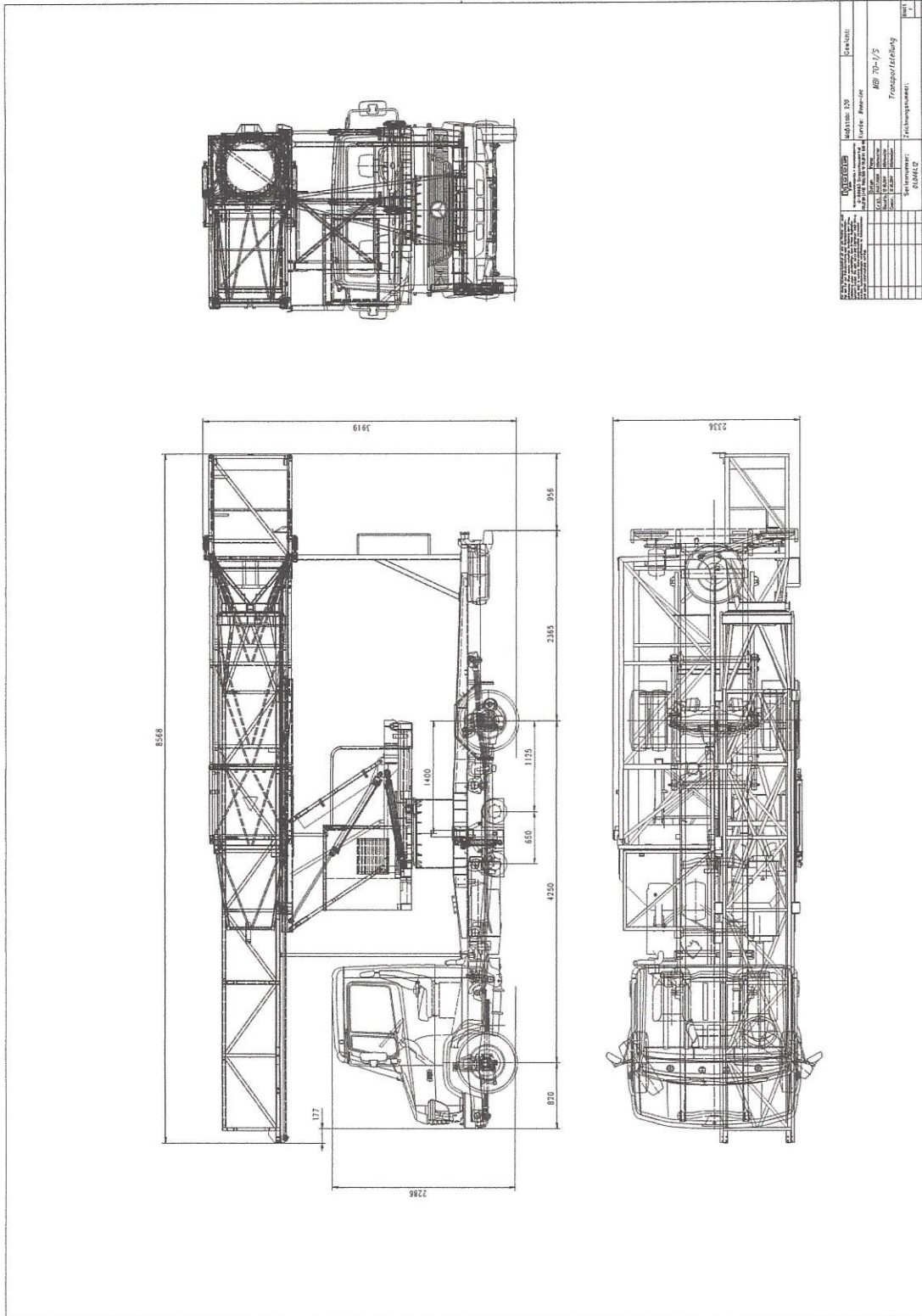
Picture 2: transport position of MBI 70-1/S truck version - subject to change
